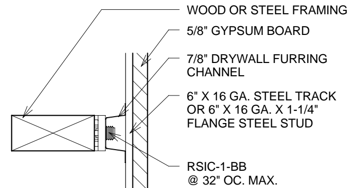
3 ENLARGED DETAIL 3" = 1'-0"
