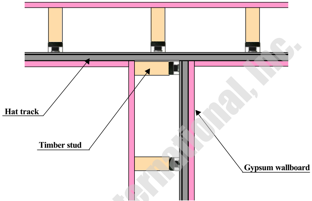
Wall Intersection
