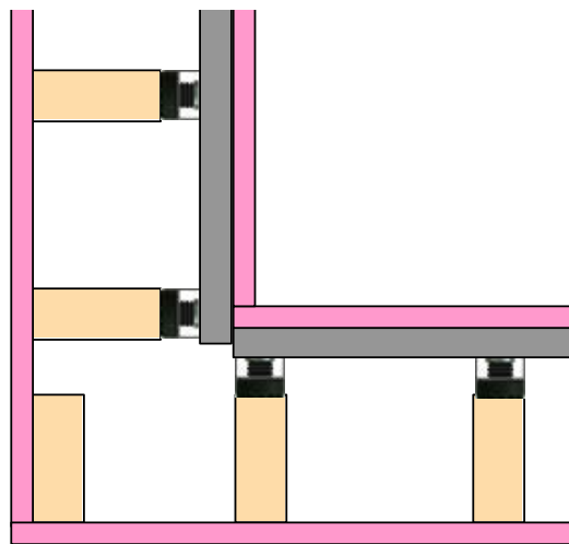
Corner Junction
