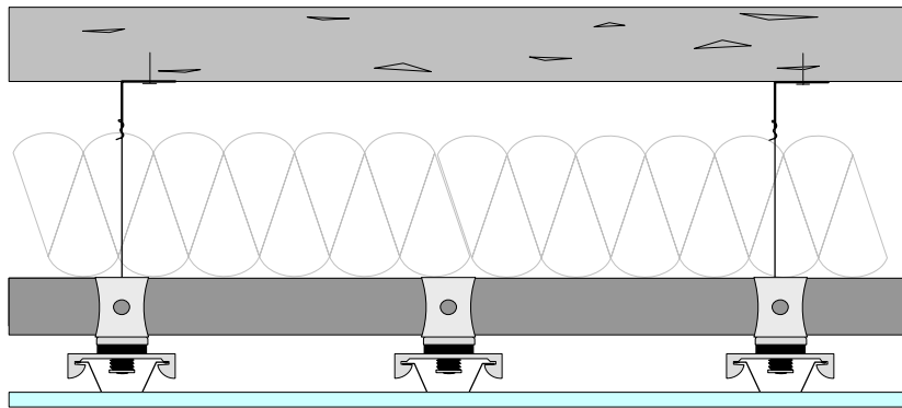
FCS RSIC1.5CRC Dropped Ceiling
