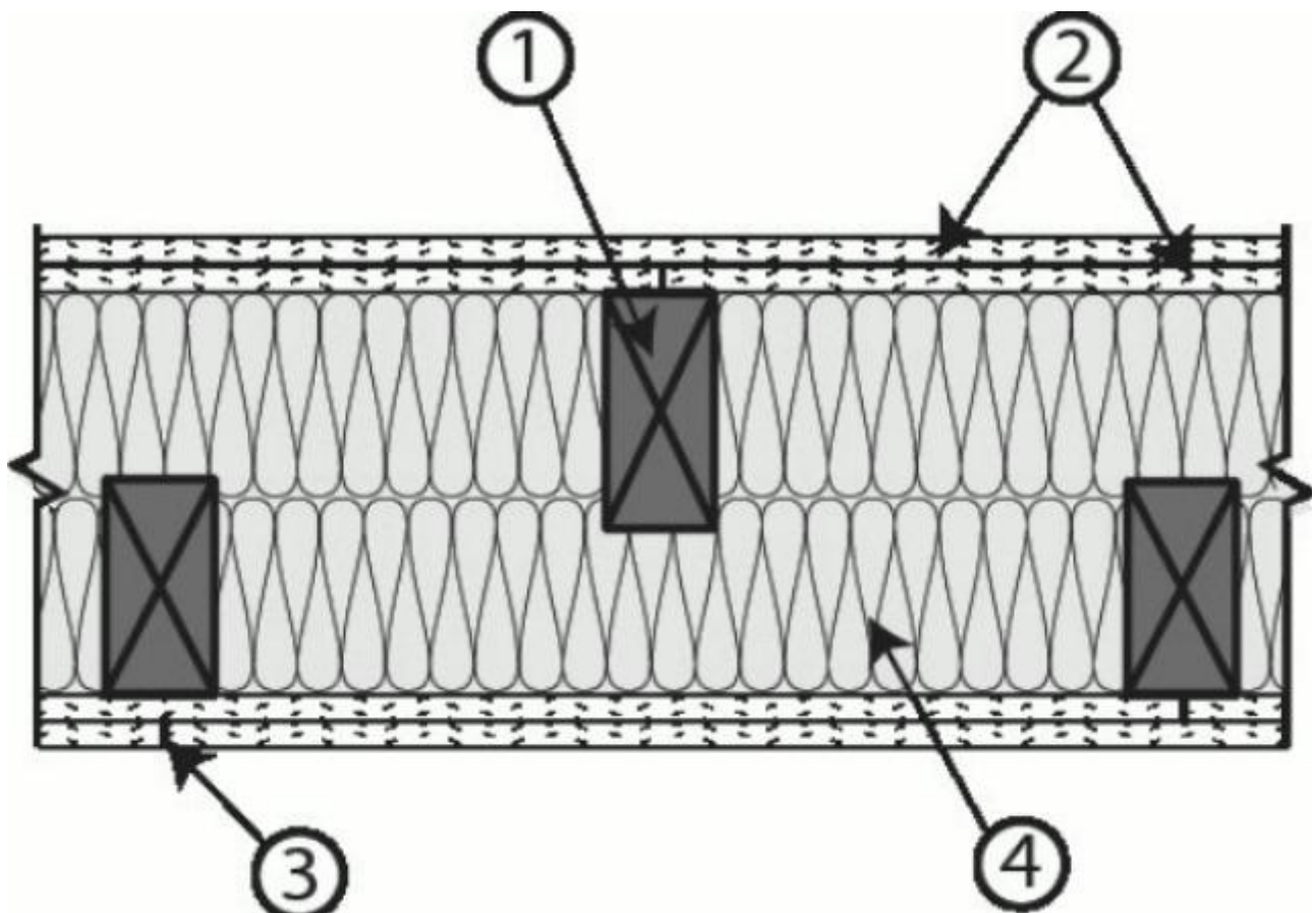
HORIZONTAL SECTION
